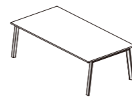
HUO-H1 1000W x 1000D x 750H/mm 2000W x 1000D x 750H/mm 2400W x 1200D x 750H/mm
